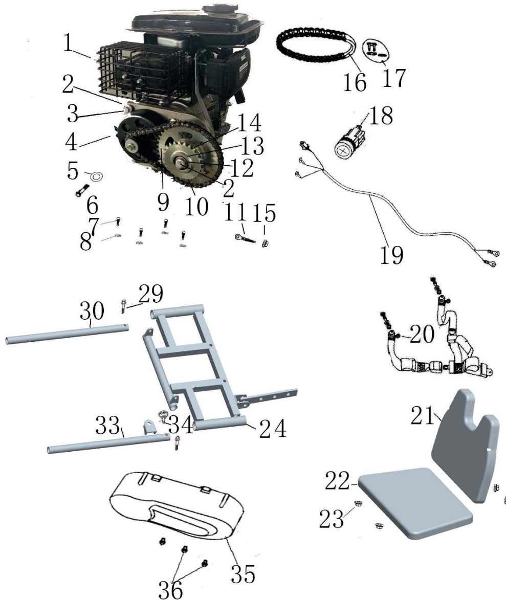
FIG. 6 ENGINE / WIRE HARNESS / ELECTRIC / SEAT
